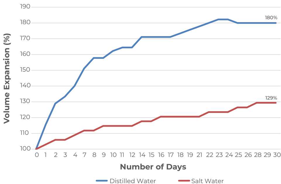
Figure 1 : Expansion rate properties of Superstop® 47B in various solutions
