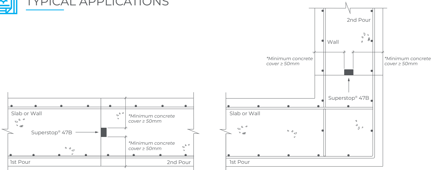
SLAB ON GROUND OR WALL SLAB TO KICKER IN WALL
